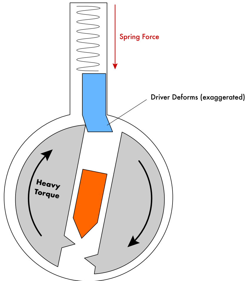
Figure 9.2: Driver pin false set by elastic deformation
