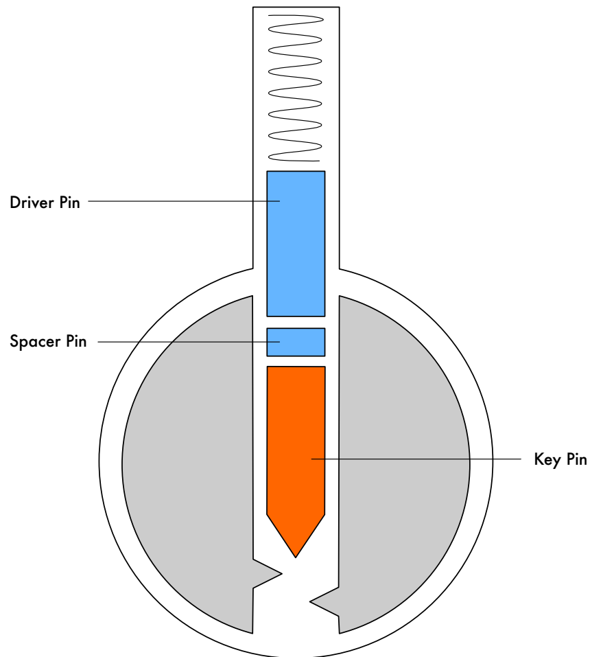
Figure 9.8: Spacer pins for master keying
