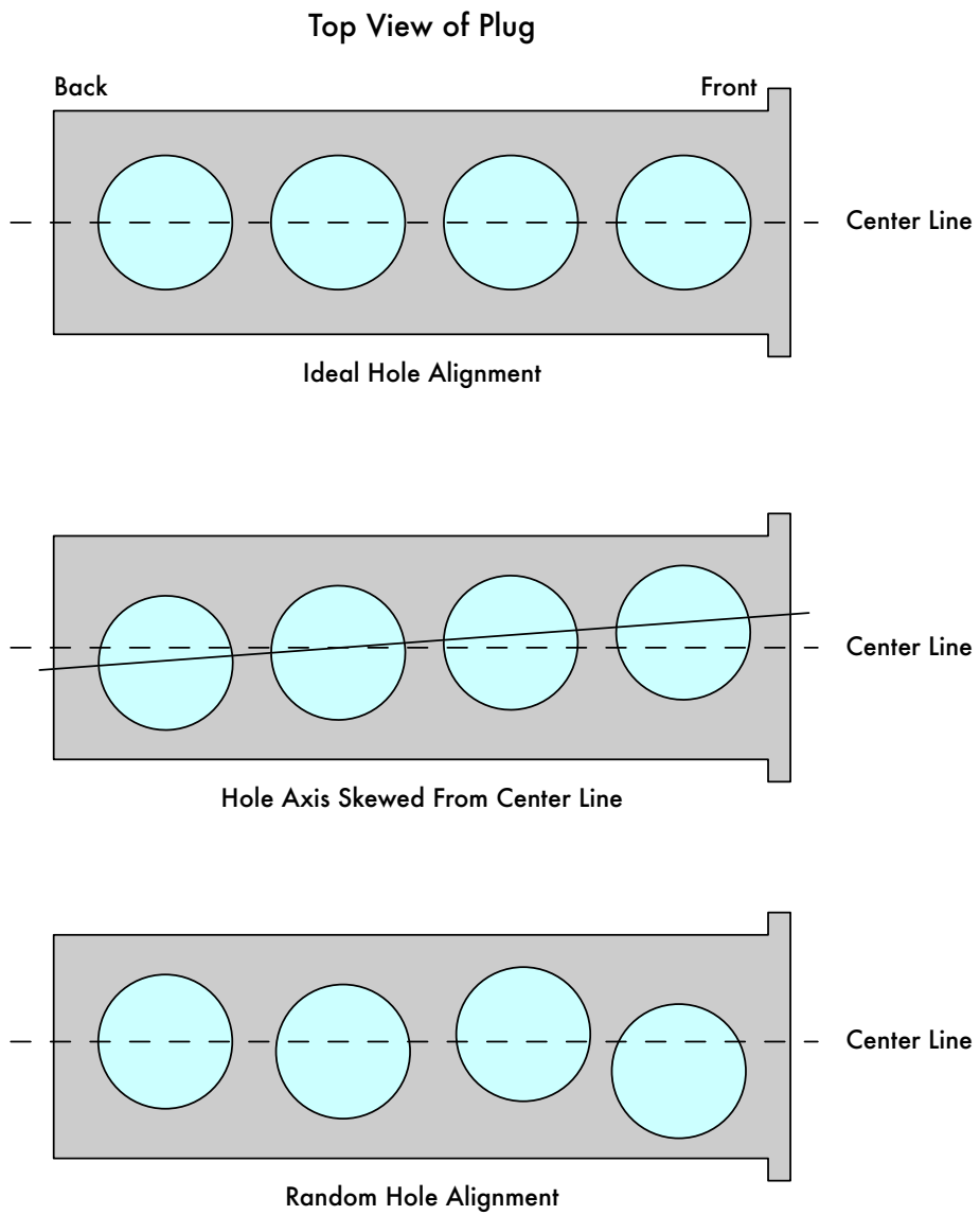
Figure 6.2: Alignment of plug holes
