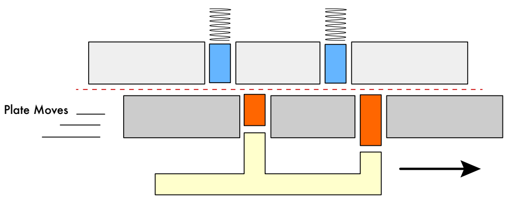
Figure 3.3 - (b) Proper key allows plate to slide
