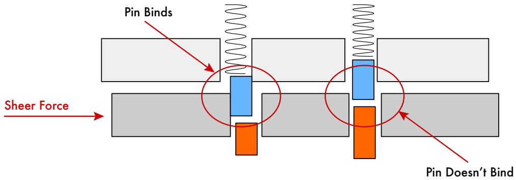
Figure 4.1 - (a) Shear force causes driver to bind
