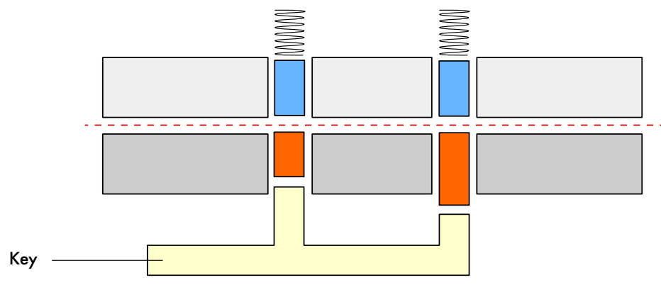
Figure 3.2 - (a) Flatland key raises pins
