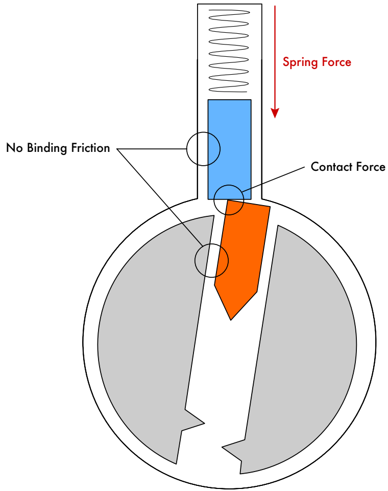
Figure 5.3 – Pins at the shear line
