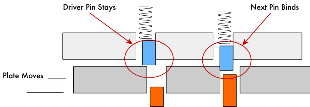
Figure 4.3 - (c) Left driver sets and then right driver binds
