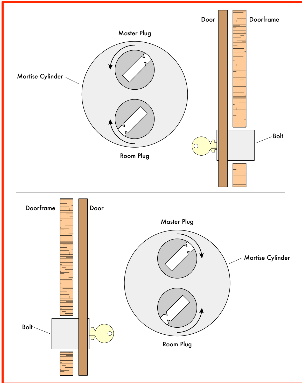
Figure 9.1: Direction to turn plug
