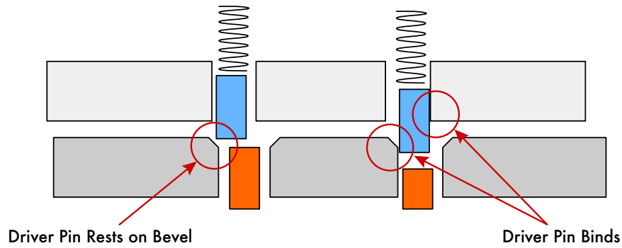
Figure 9.6: (a) Driver sets on bevel
