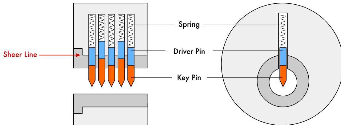
Figure 2.1: Workings of pin tumbler locks
