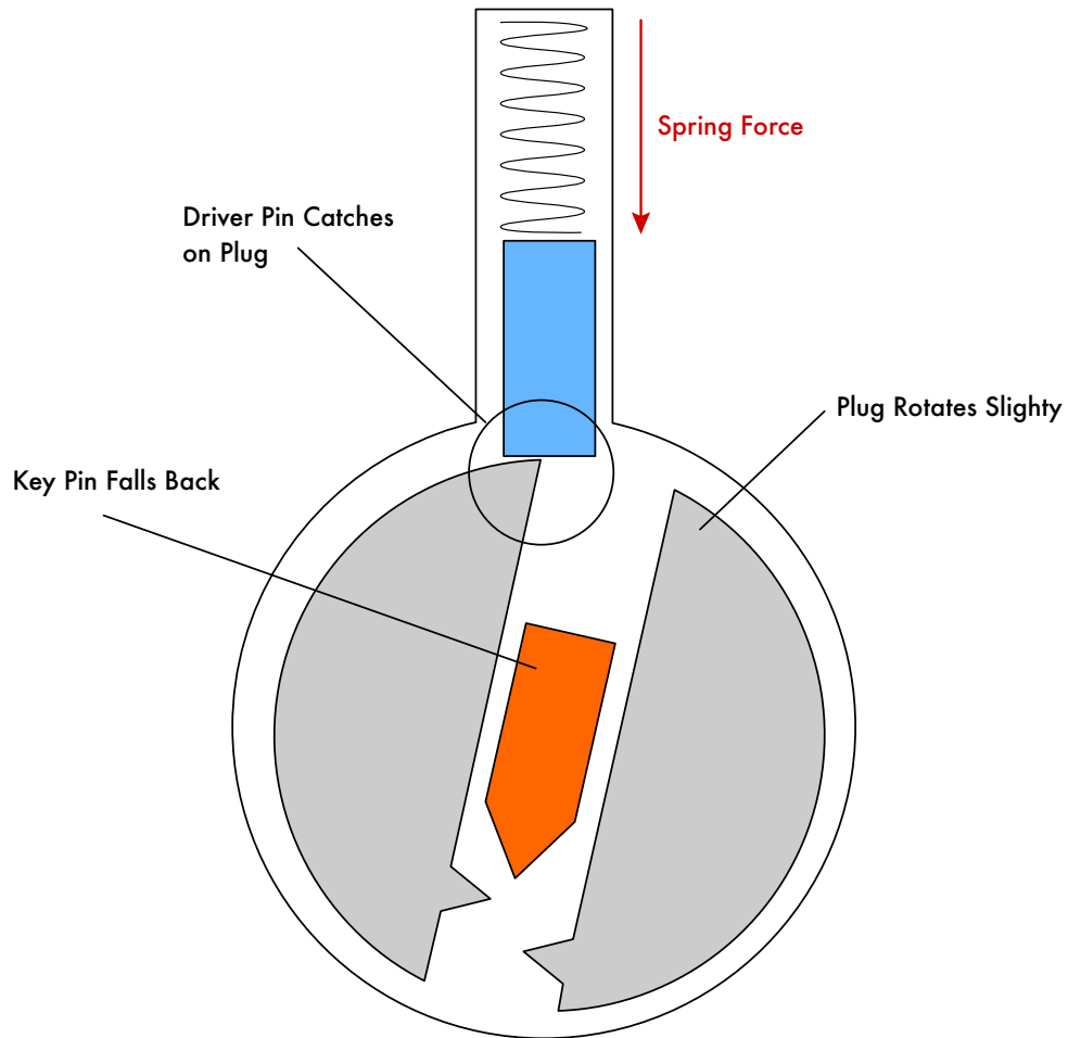
Figure 6.1: Driver pin catches on plug
