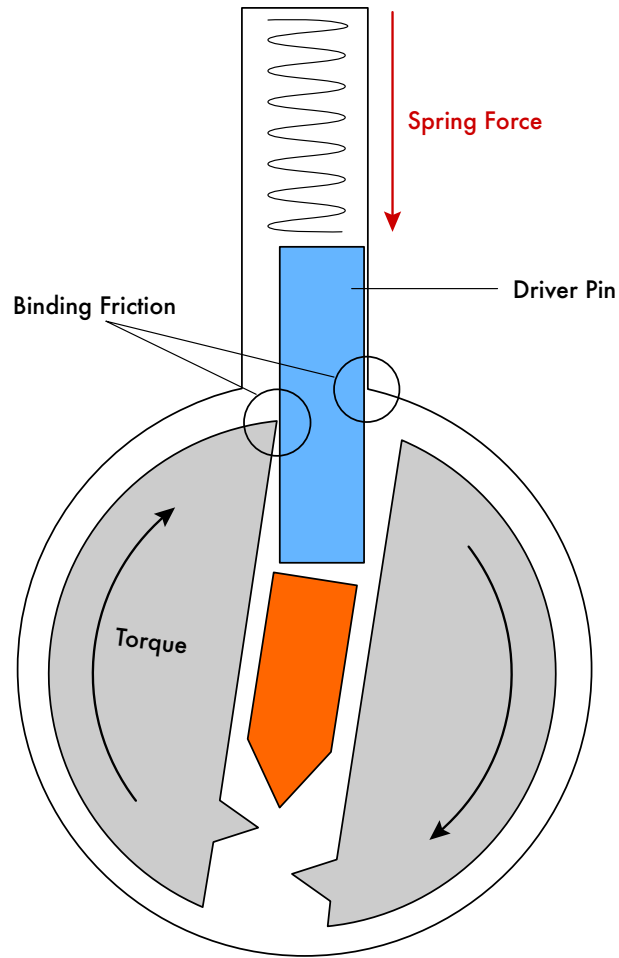
Figure 5.2 – Binding in the pin-column model
