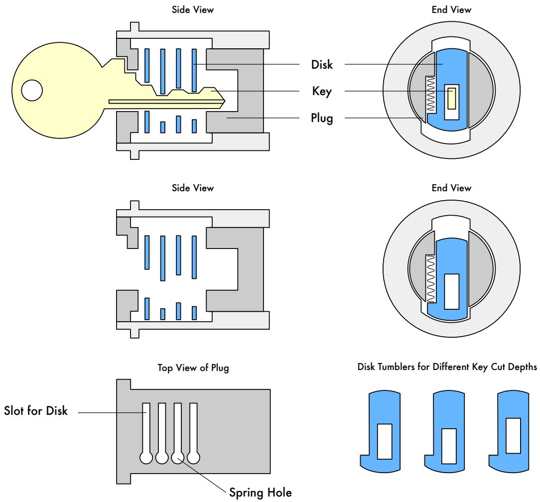
Figure 9.10: Workings of a disk tumbler lock
