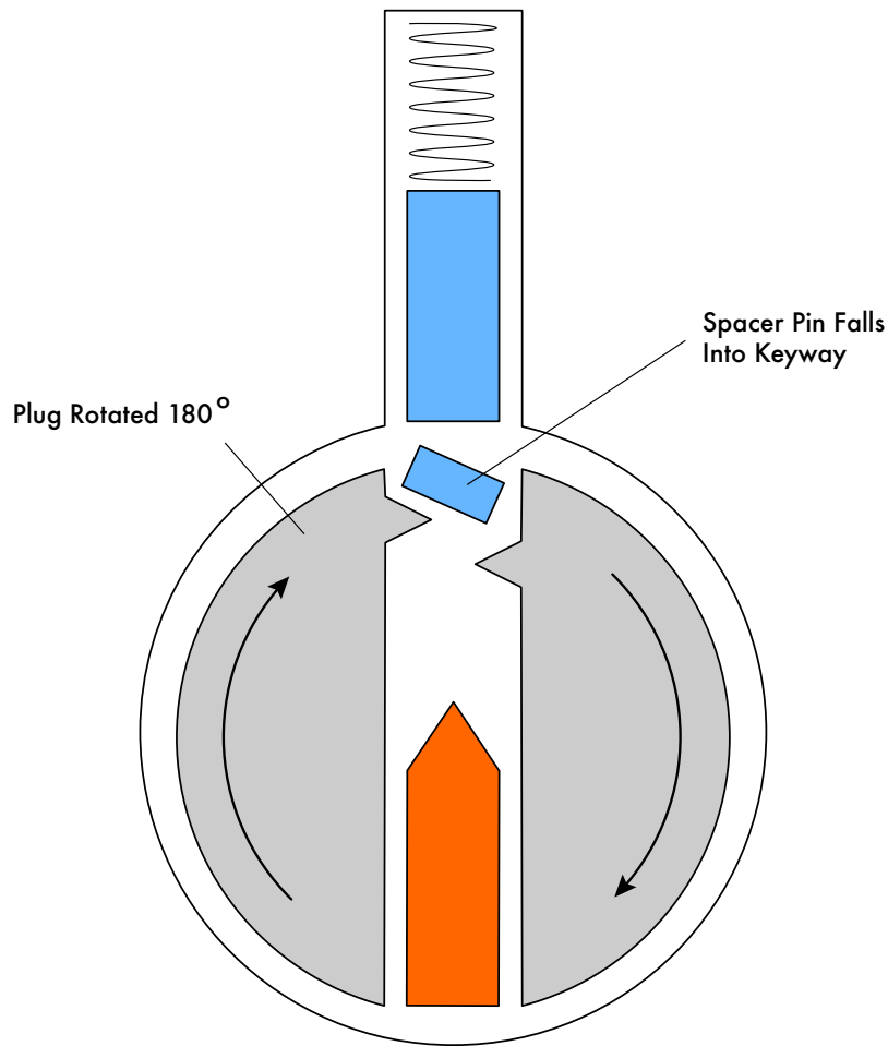
Figure 9.9: Spacer or driver pins can enter keyway
