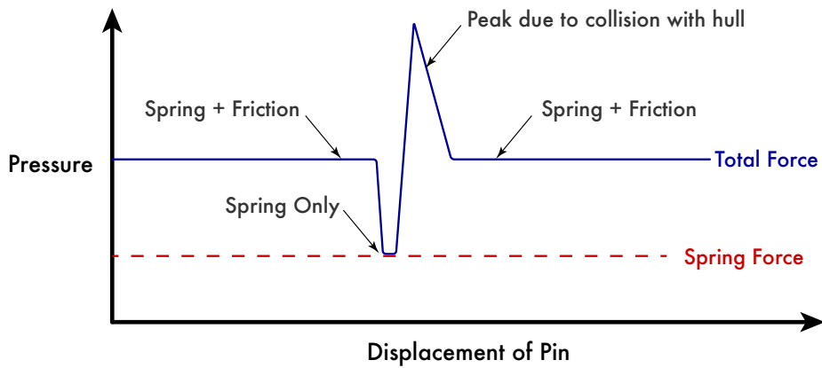
Figure 5.5 – Pressure required to move pins
