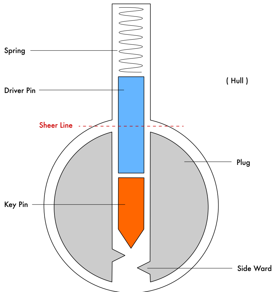
Figure 5.1 – The pin-column model
