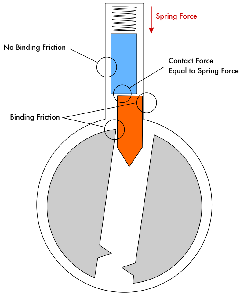
Figure 5.4 – Key pin enters the hull
