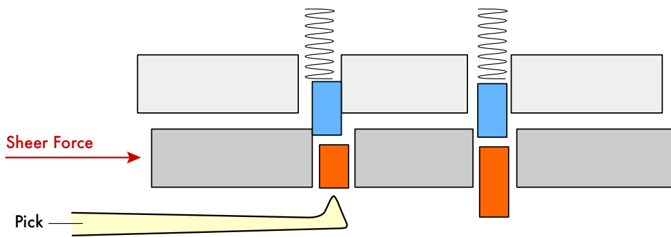
Figure 4.2 - (b) Pick lifts the binding key
