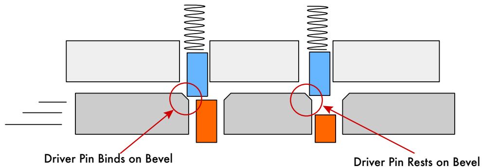
Figure 9.6: (b) Driver jams on bevel
