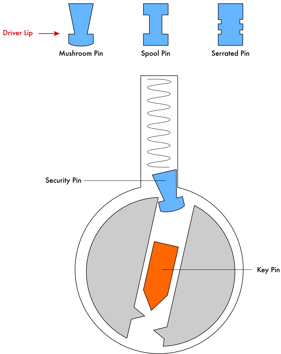
Figure 9.7: Mushroom, spool, and serrated pins
