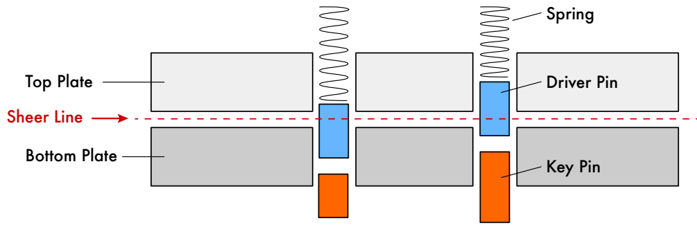
Figure 3.1 - Flatland model of a lock
