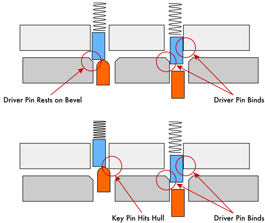
Figure 9.4: Beveled plug holes and rounded key pins
