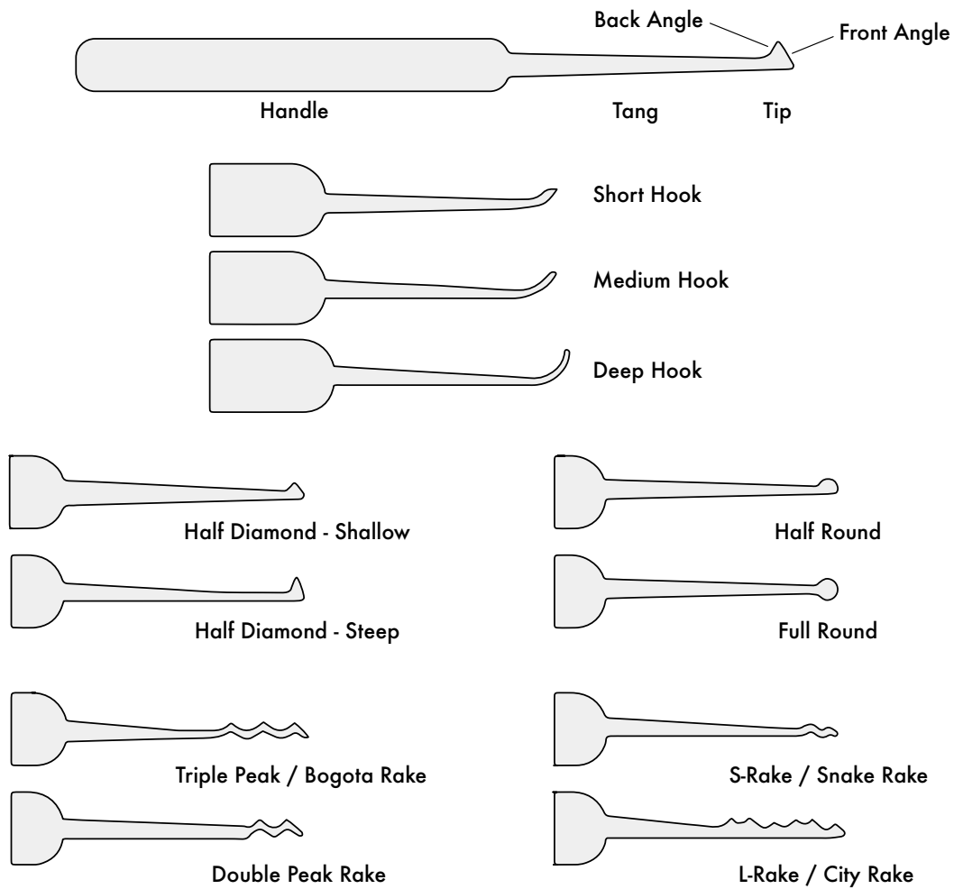
Figure A.1: Selection of pick shapes
